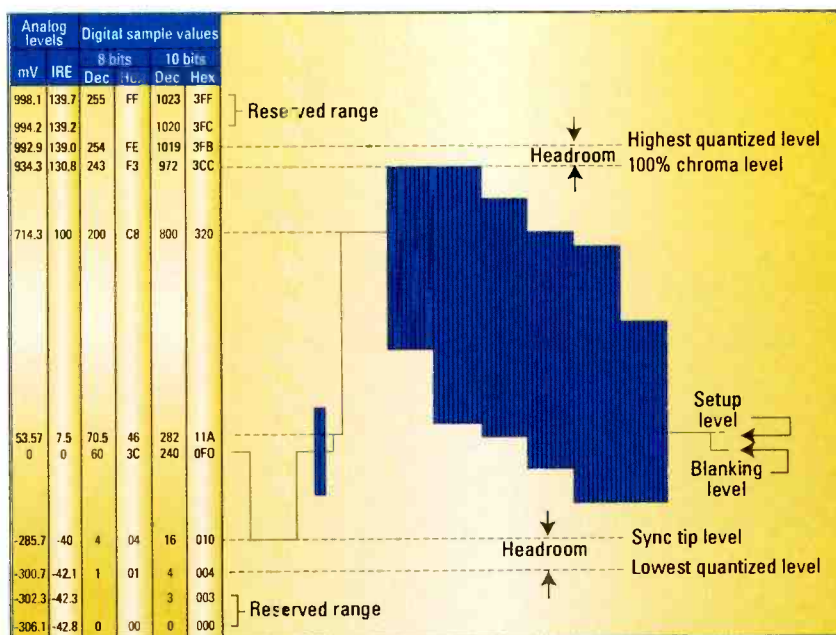
Figure 7. Relationship between analog signal levels and digital sample values
