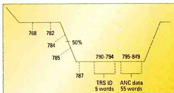
Figure 6. 4f_{sc} NTSC horizontal sync period details showing location of TRS-ID and optional ancillary data
